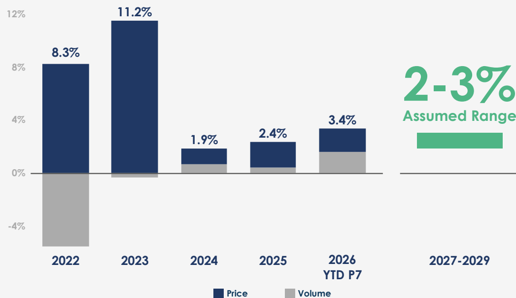
Category Growth
